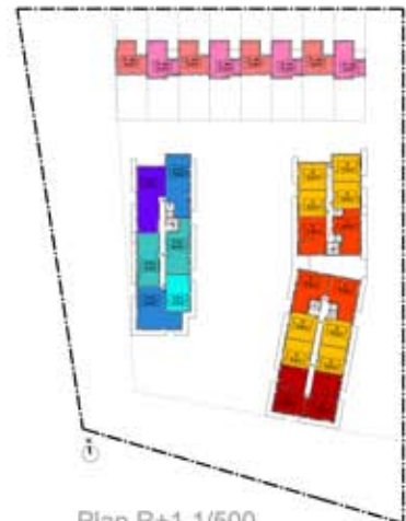
Plan R+1 1/500
